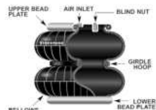
CONVOLUTED AIR SPRINGS WITH CRIMPED BEAD PLATES
