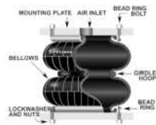
CONVOLUTED AIR SPRINGS WITH STEEL BEAD RINGS
